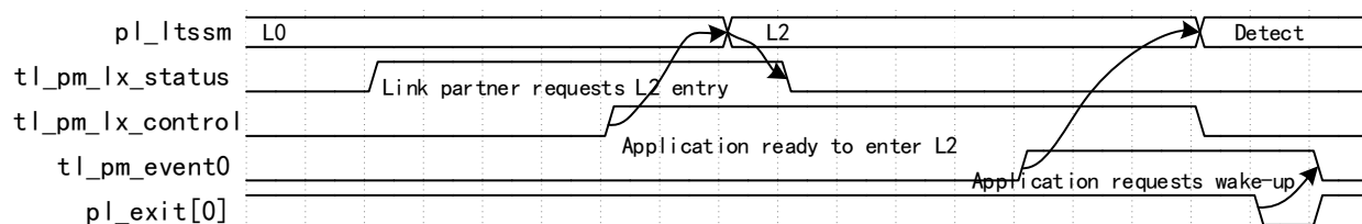
图 2-34 L2 Entry from Upstream Port
