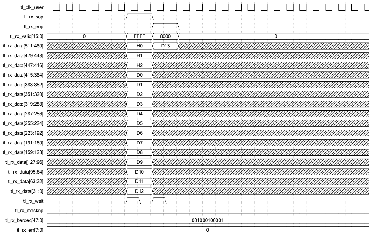
图 2-19 接收 3DW Header With 14DW Payload
