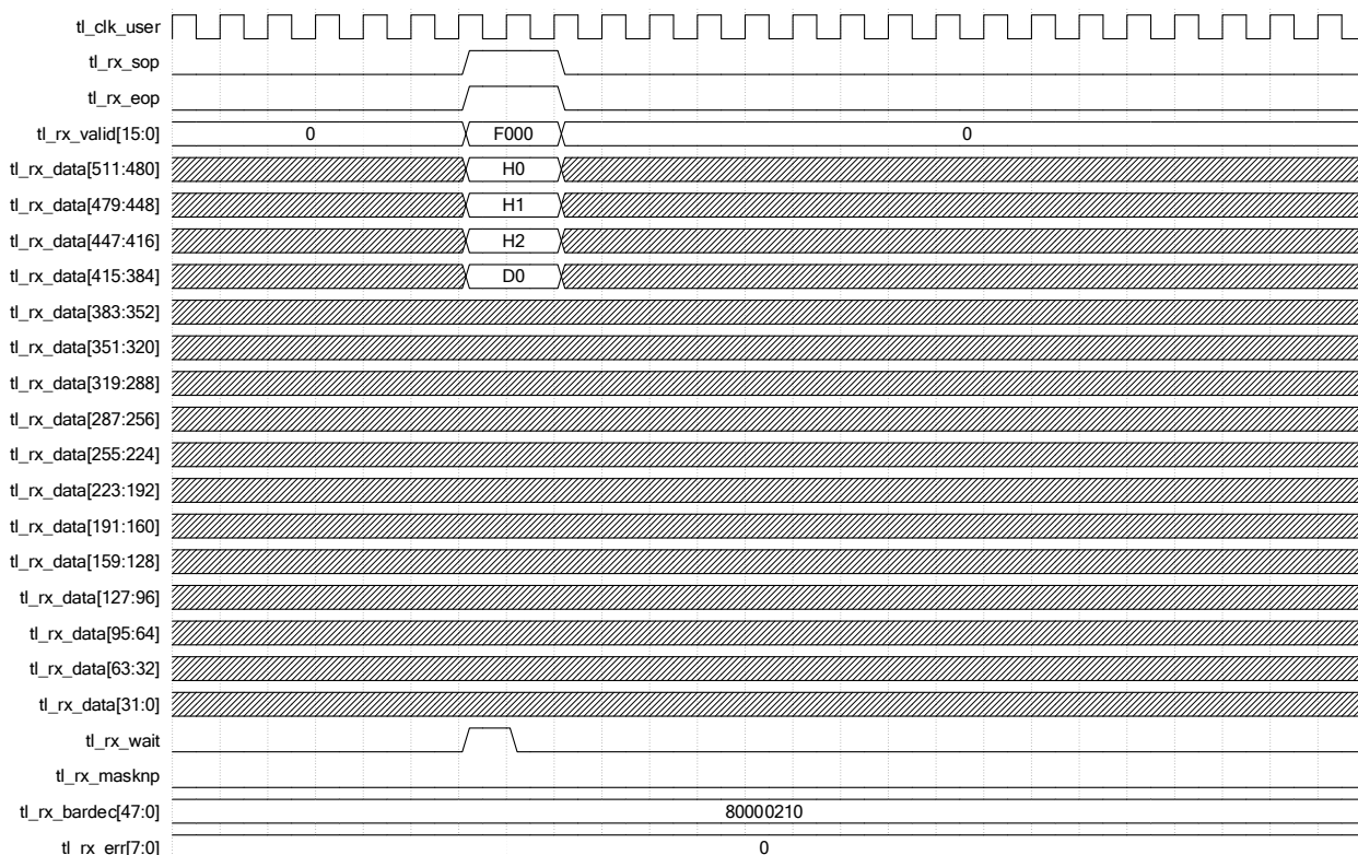
图 2-18 接收 3DW Header With 1DW Payload
