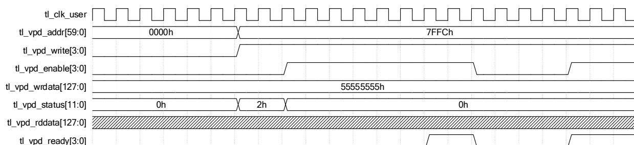
图 2-40 VPD Write with Wait
