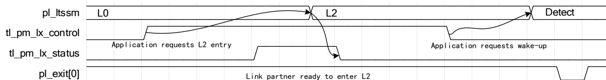
图 2-33 L2 Entry from Downstream Port
