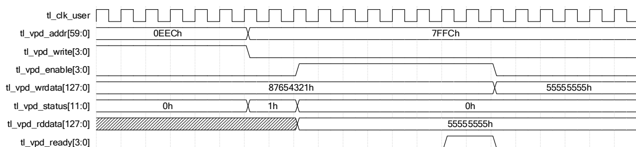
图 2-39 VPD Read with Wait
