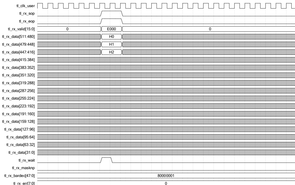
图 2-17 接收 3DW Header Without Payload
